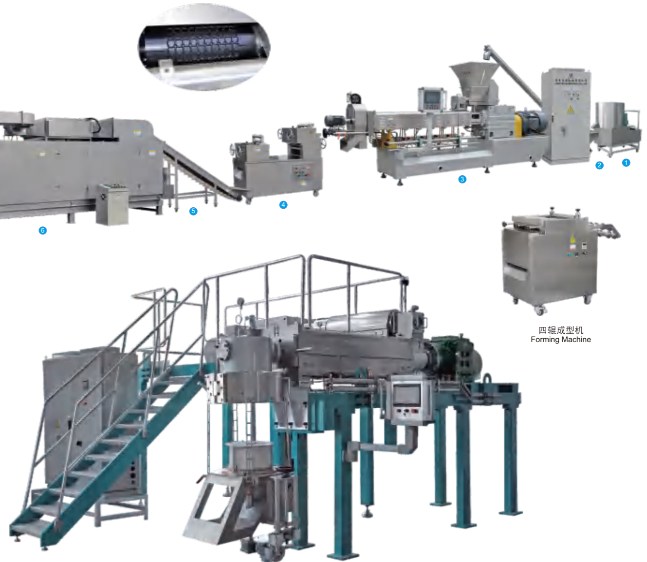
胚料二次膨化类产品挤压机 Cooking and Forming Extrusion System
