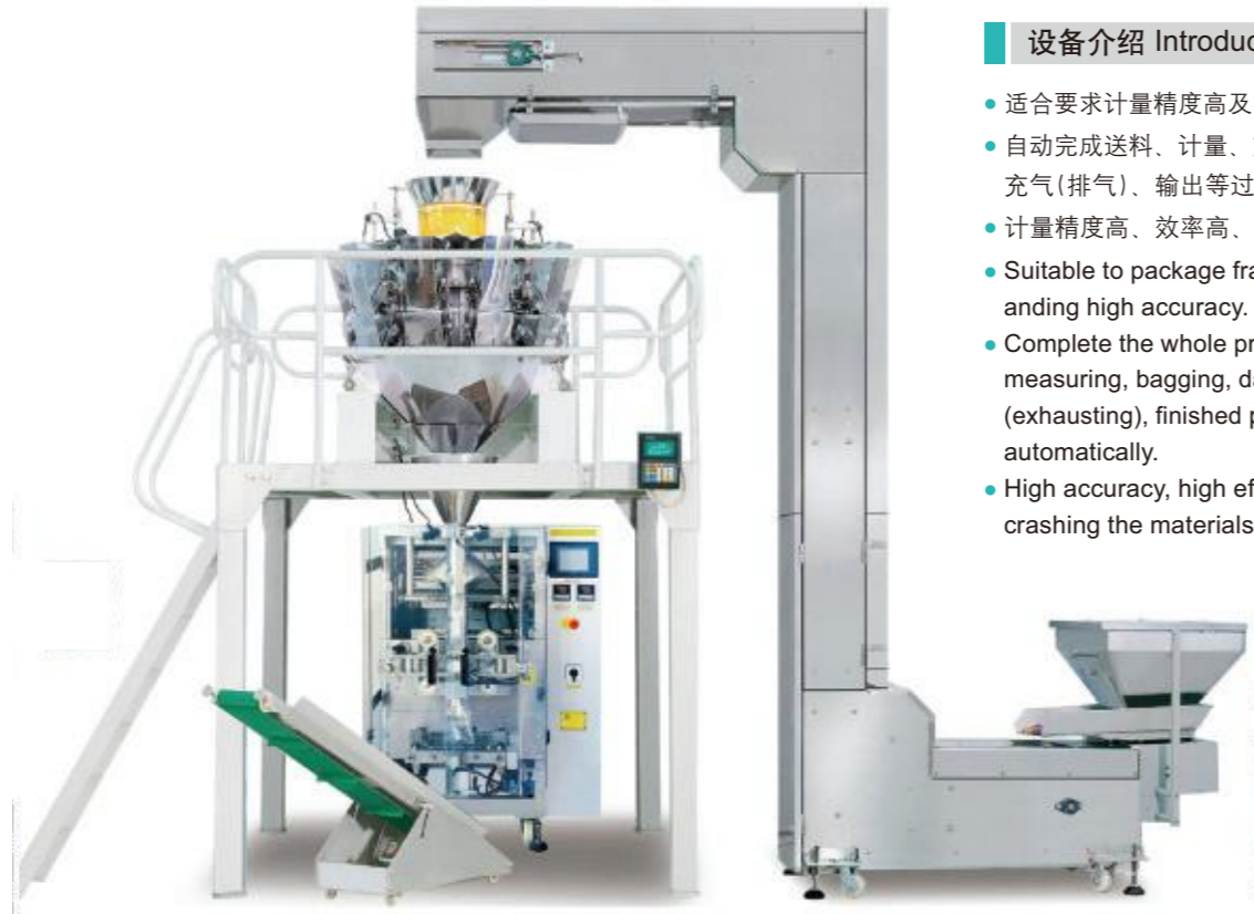
大型立式全自动包装机配套系列 Large-sized Vertical Automatic Packing Machine Series
